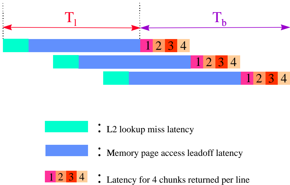
Figure F-1 Pentium® II and Pentium III Processors Memory Pipeline Sketch
