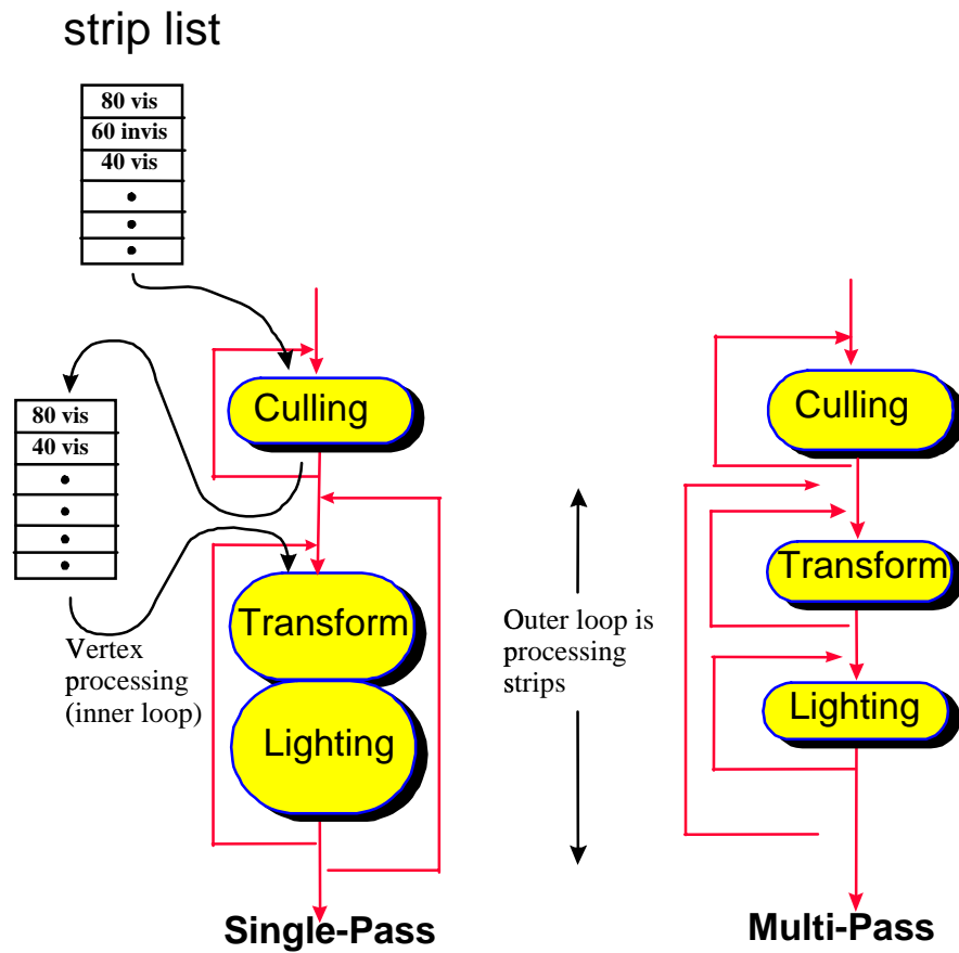
Figure 6-6 Single-Pass vs. Multi-Pass 3D Geometry Engines
