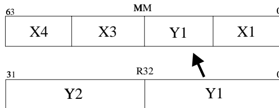
Example 4-16 pinsrw Instruction Code
