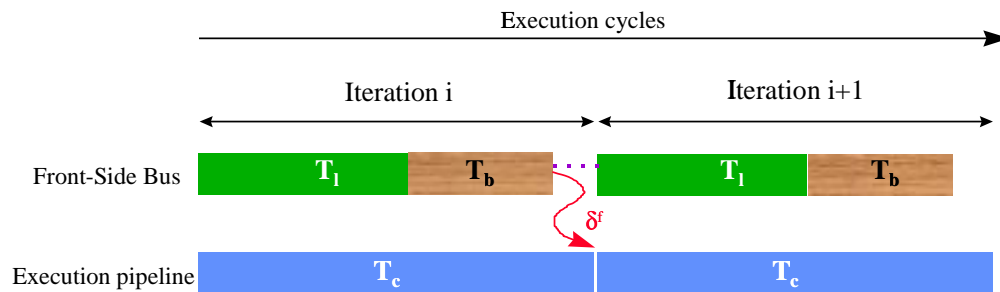
Figure F-3 Compute Bound Execution Pipeline
