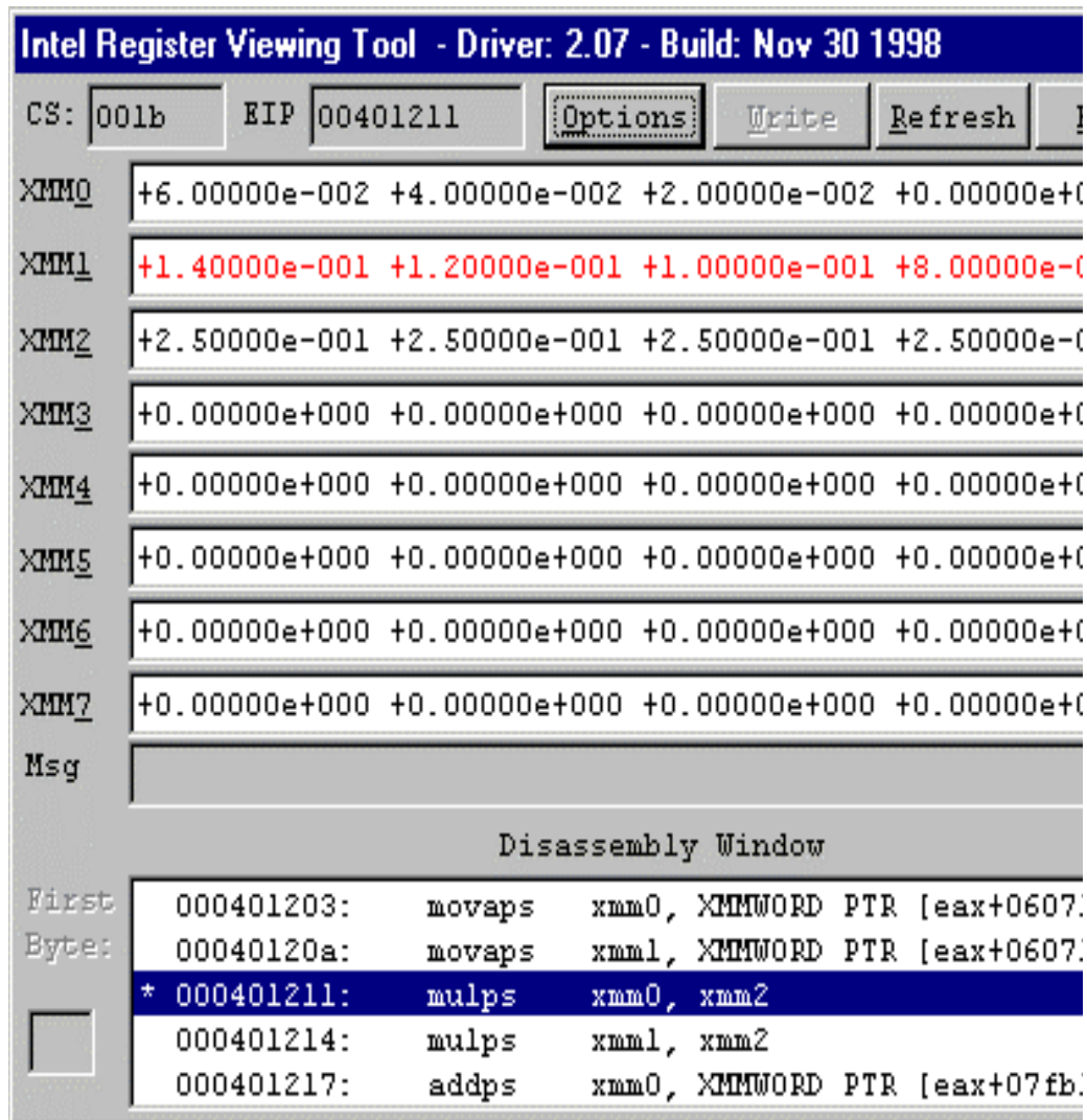
Figure 7-5 The RVT: Registers and Disassembly Window
