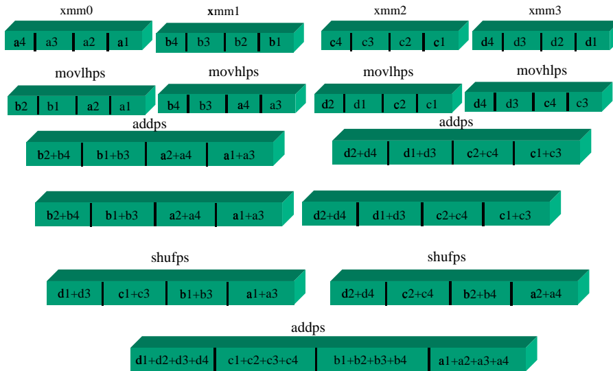
Figure 5-2 Horizontal Add Using movhlps/movhps
